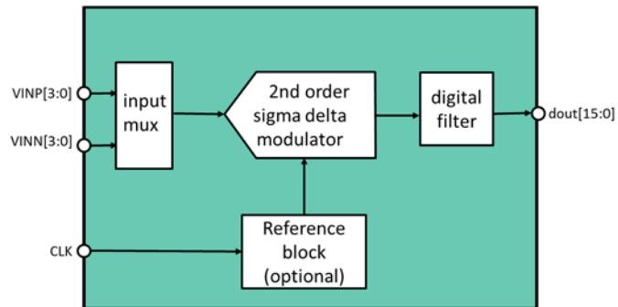
Fig. 1: IP-Level Block Diagram
